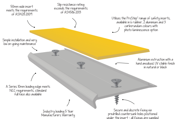
A SERIES 10MM FACE (NCC COMPLIANT) UM002A
