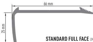
STANDARD FULL FACE UM002
