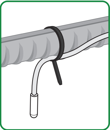
6 Secure the cable and temperature probe below the rebar
